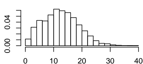
Density of gwesp.fixed.0
