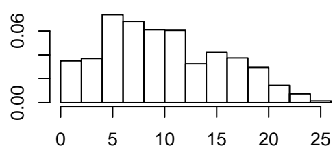
Density of edges
