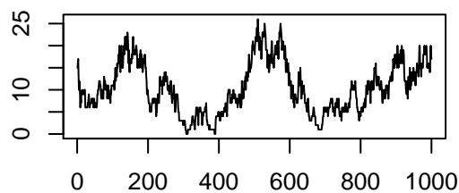
Trace of edges
