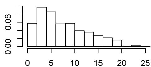
Density of gwesp.fixed.0
