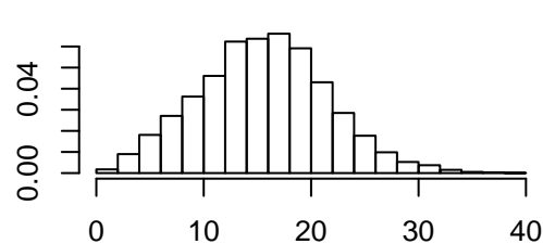
Density of edges
